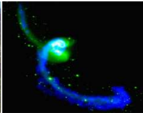
A radio image of the interacting Antennae galaxies
