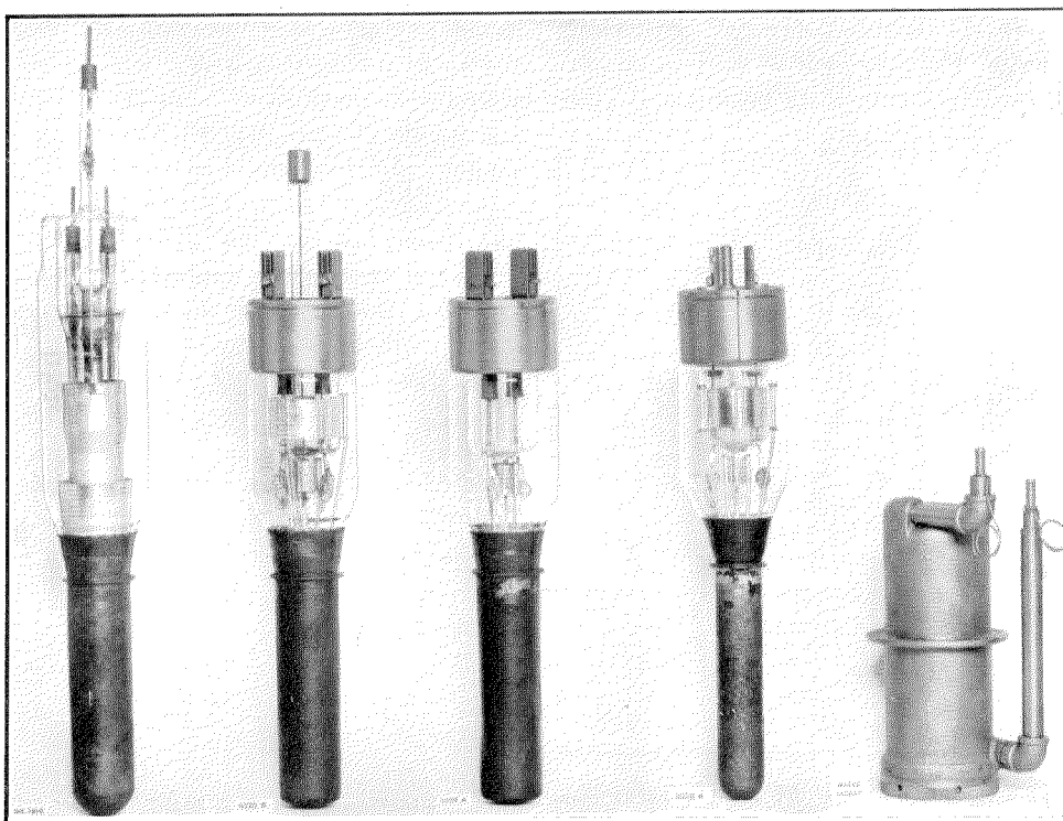
Figure 13—The Water-cooled Group.
