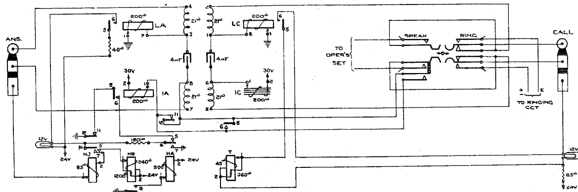
Figure 7—Universal Cord Circuit.
