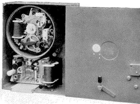
Figure 4—Inside Box of Succession Fire Alarm Box.
