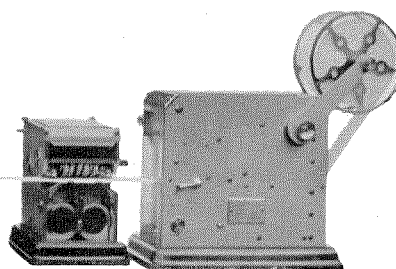
Figure 13—Register, Time Stamp and Take-up Reel as Mounted at Fire Station.
