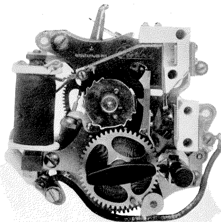
Figure 5—Succession Non-interfering Box Movement.
