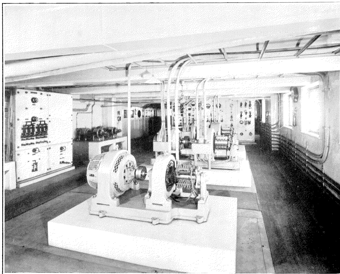
Figure 3—The Power Plant.
