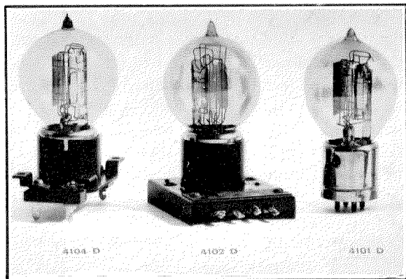
Figure 3—The Repeater Group.
