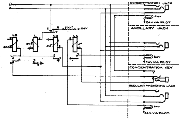
Figure 19—Incoming Jack-ended Junctions from Manual Exchanges.
